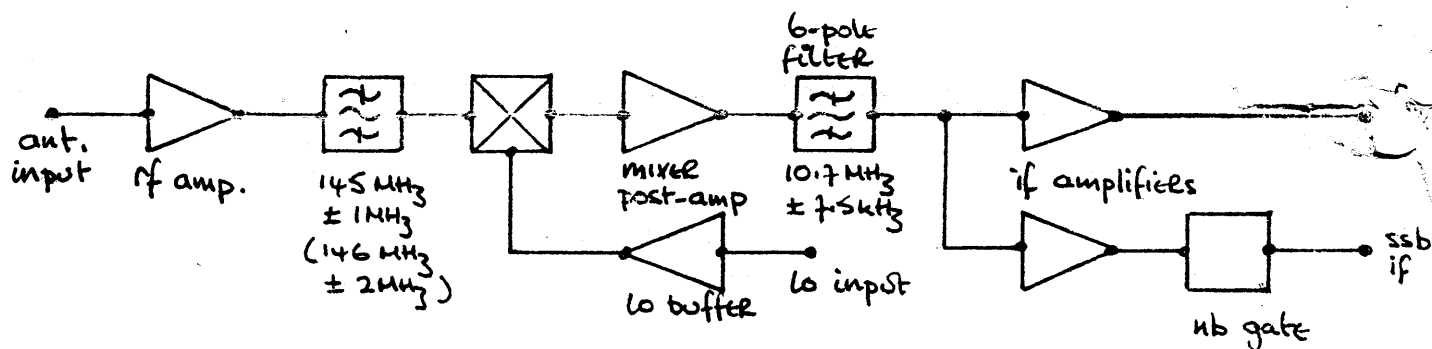
Block schematic.
