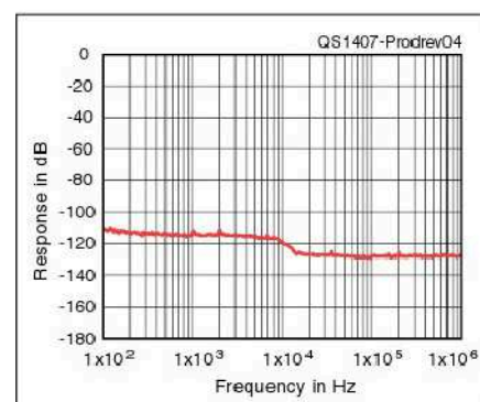
Figure 4 — Spectral display of the Icom IC-7100 transmitter output during composite-noise testing. Power output is 100 W on the 14 MHz band. The carrier, off the left edge of the plot, is not shown. This plot shows composite transmitted noise 100 Hz to 1 MHz from the carrier. The reference level is 0 dBc, and the vertical scale is in dB.
